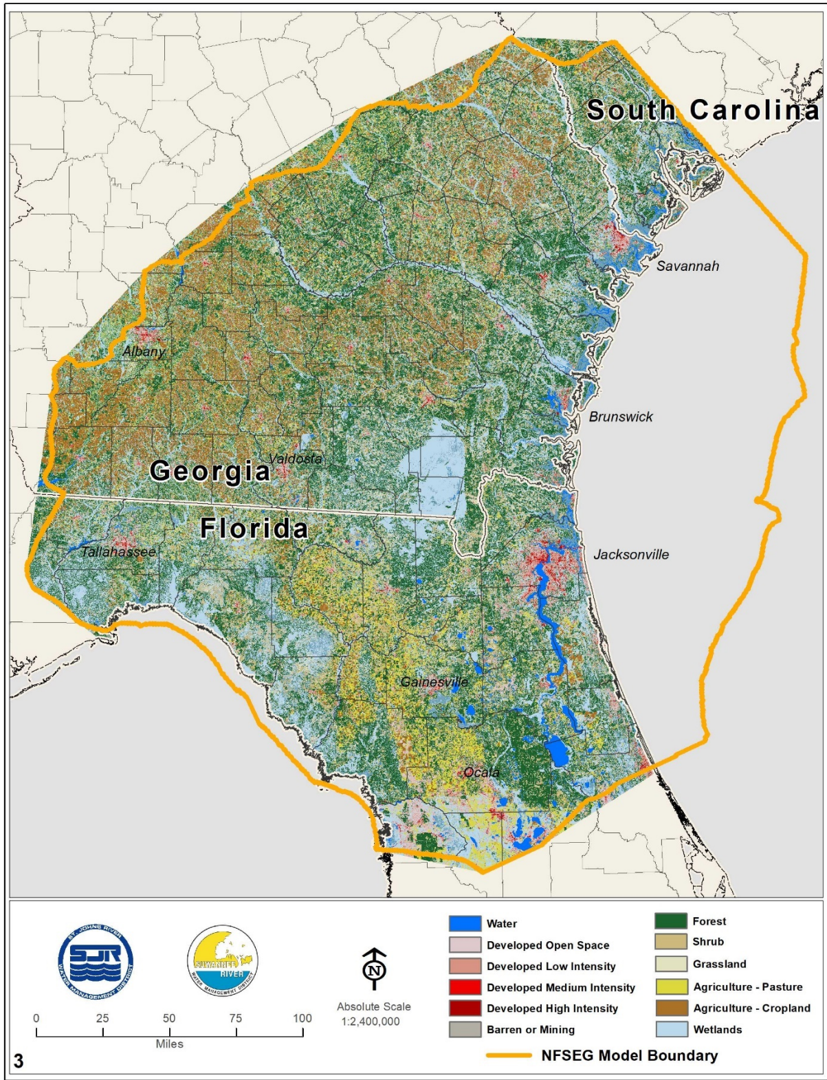
Figure 1-3. Land-Use Coverage
